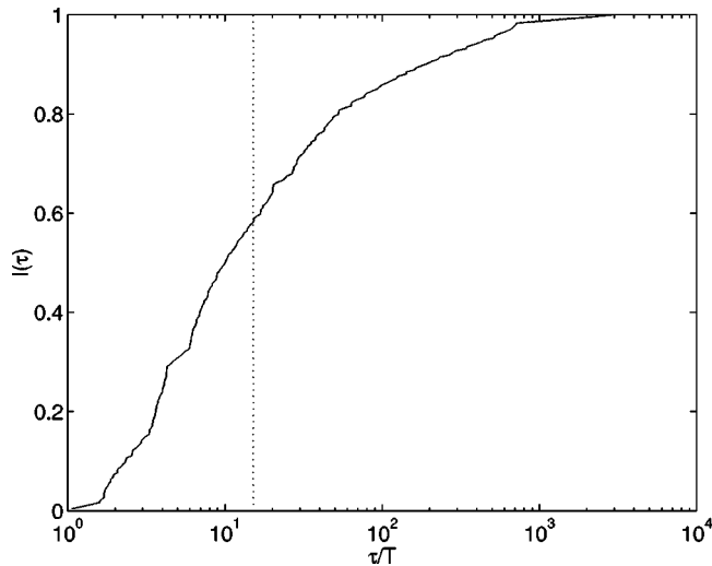
FIG. 4. Integrated distribution function for the decay times \tau_{\text{qu}} = \hbar/2 \text{Im}[\lambda_l(k)] of the quantum metastable states for the parameters of Fig. 3. The vertical line shows the value of the classical decay time \tau_{\text{cl}} = 15.2 T .
