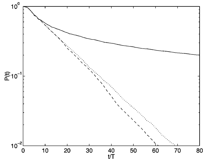
FIG. 5. Probability for a classical and quantum particle to stay within the chaotic component |p| < 1.8 ( \omega = 0.3 , F \approx 0.02 ). Dotted line: classical result, solid line: quantum result provided the condition T_B = T_\omega ( \hbar = 0.5 ), dashed line: “incommensurate” case ( \hbar = 0.5109531 ). In the quantum case the curves were obtained by simulating wave packet dynamics with minimal uncertainty packet centered at x=0 , p=0 as an initial condition.
