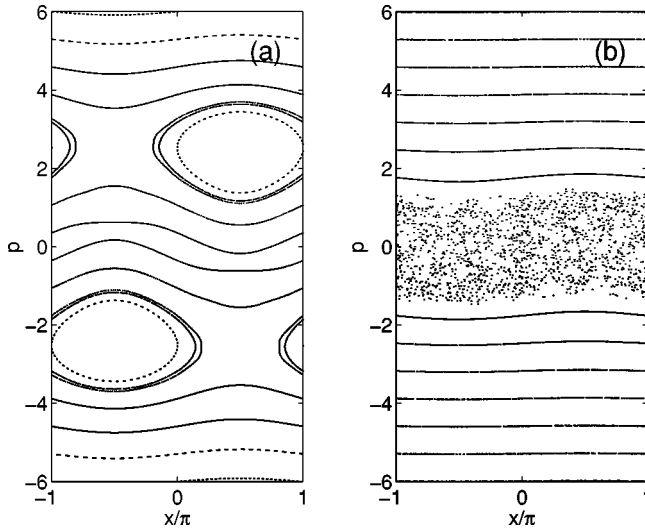
FIG. 1. Phase space portrait of the system (1) for \omega \approx 2.51 > \omega_{\text{cr}} \sim 1 (a) and \omega = 0.3 < \omega_{\text{cr}} (b). 18 different trajectories p(t_n) , x(t_n)_{\text{mod}:2\pi} , t_n = nT + T/4 are plotted in each case.
