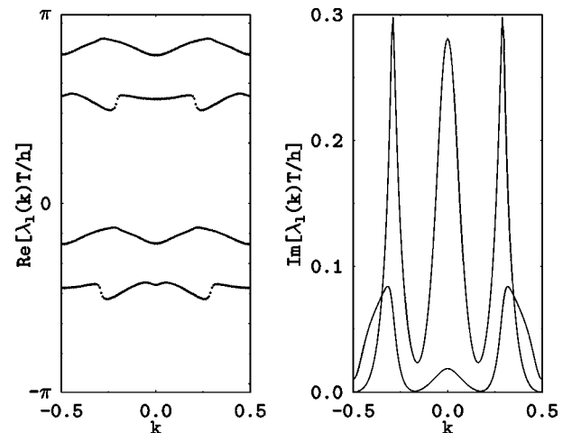
FIG. 3. Same as Fig. 2 but for \omega = 0.3 < \omega_{\text{cr}} , F = \hbar \omega/2\pi \approx 0.02 . (The imaginary part is shown only for two upper bands. For lower bands the curves should be shifted by one-half of the Brillouin zone.)
