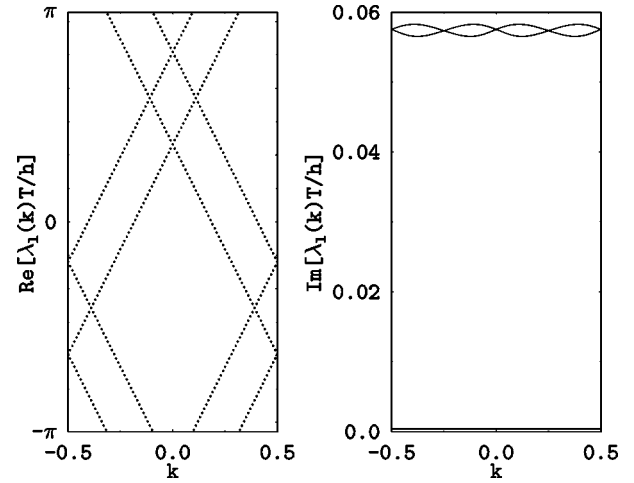
FIG. 2. Real and imaginary parts of the quasienergies corresponding to first four metastable Wannier-Bloch states of the system (1). The value of the driving frequency is \omega \approx 2.51 (scaled Planck constant \hbar = 0.5 , F = \hbar \omega/2\pi = 0.2 ).
